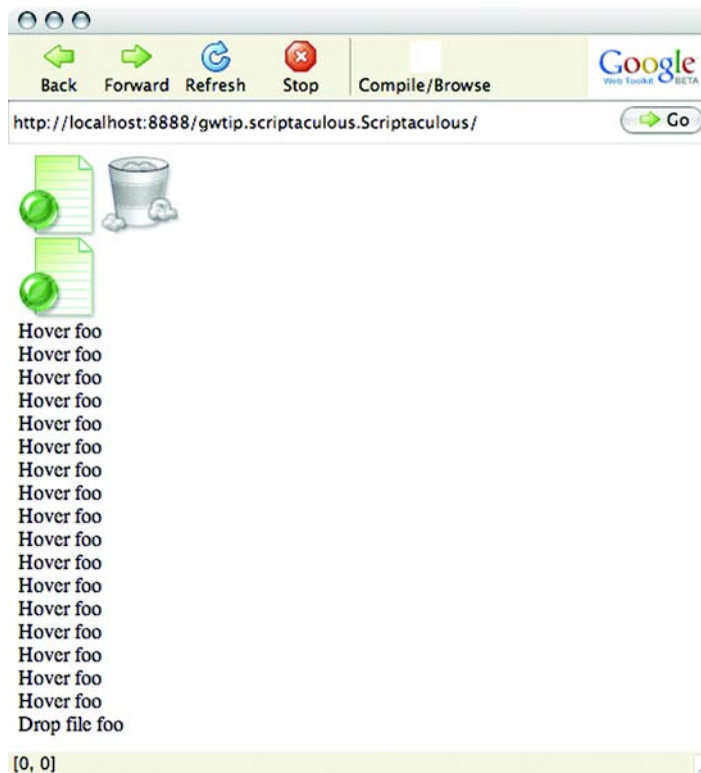
Figure 6.8 Removing one of three file icons by dragging it to the trash and dropping it. Notice the hover events followed by the drop event as a file icon is dragged and dropped onto the trash can. (Icons courtesy of kellishaver.com.)
