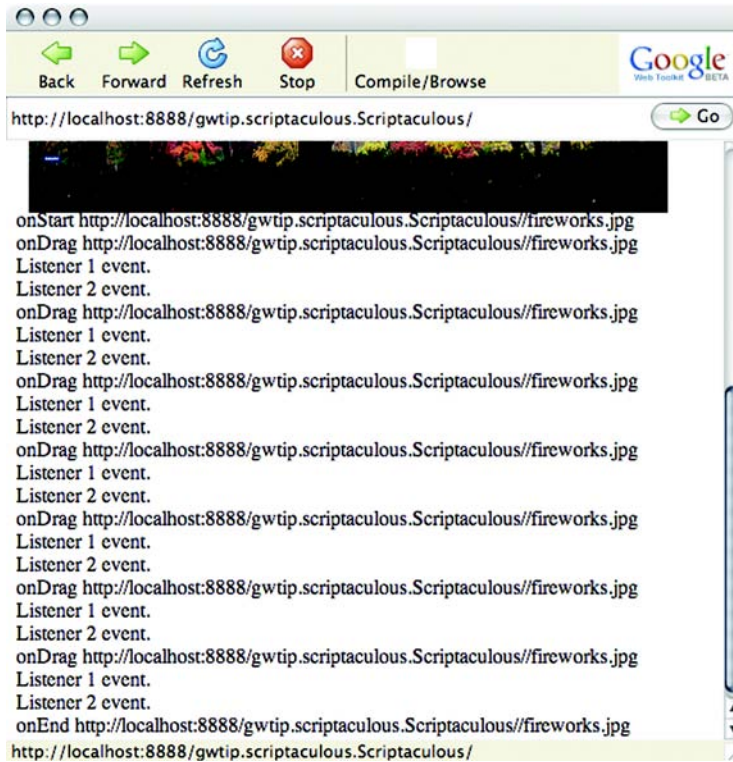
Figure 6.7 DragListeners and DragObservers fired through a drag. Here we see the DragObserver events firing, followed by the DragEvents we saw in the previous section. Notice that the observers see onStart() and onDrag() , and not just the basic event.
