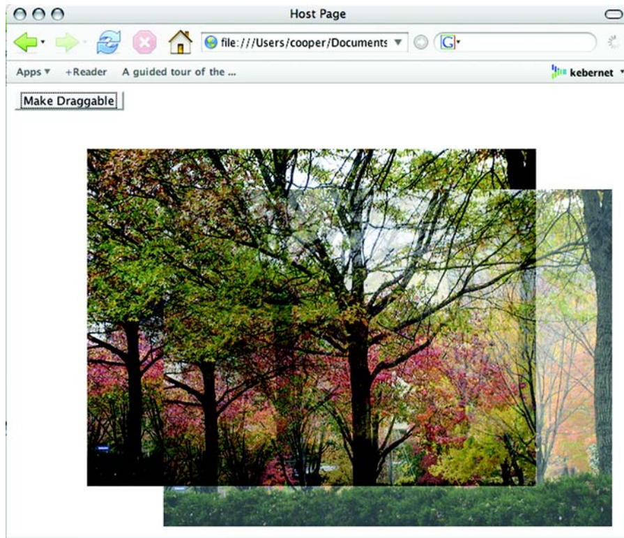
Figure 6.5 Dragging the image around in the window creates a ghost image as a placeholder. When the image is dragged, a partially transparent copy will follow the mouse.
